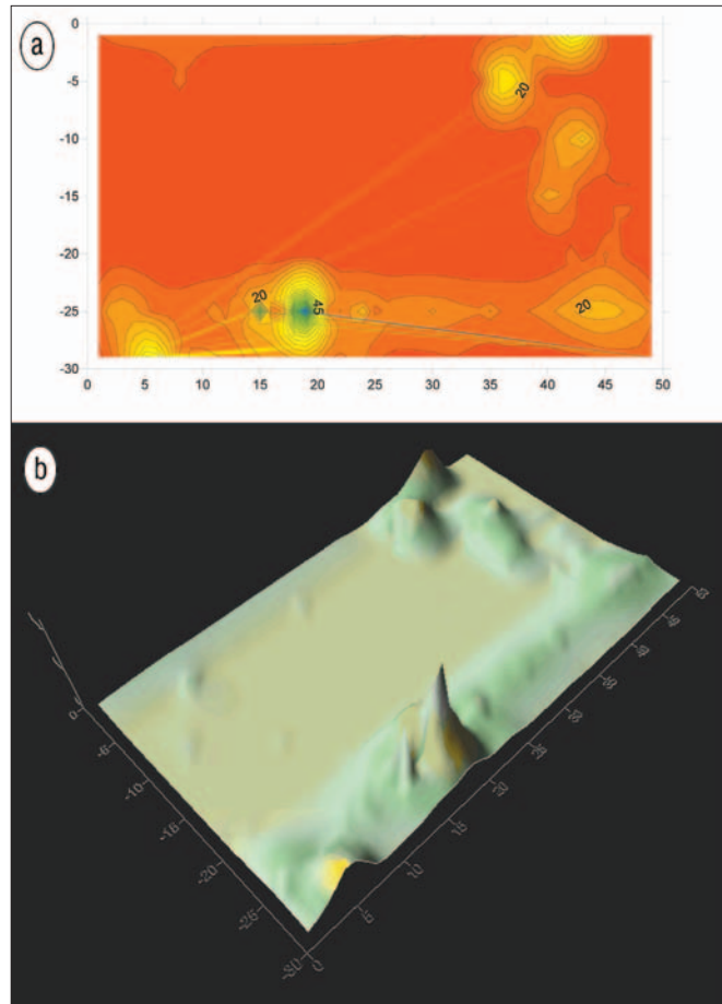
Figure 5. A 2D and 3D EM image of the study area based on the magnetic susceptibility response at a source frequency of 24 570 Hz. The data pinpointing the abandoned well (largest peak) connected to a legacy pipeline, suggesting that this was once a producing oil/gas well.
