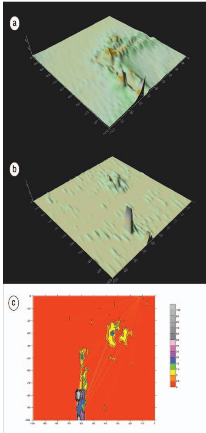
Figure 8. (a) The electrical conductivity properties based on a source frequency of 25 080 Hz shows a buried pipeline making a 90^\circ turn. (b) By examining a different EM profile based on the magnetic susceptibility properties with a source frequency of 1530 Hz, the effects of the pipeline are filtered out, highlighting the location of abandoned well (middle). (c) A 2D map view of the study area is shown and a circular feature in blue (perhaps the actual well?) is evident inside the disturbed zone (bottom).
